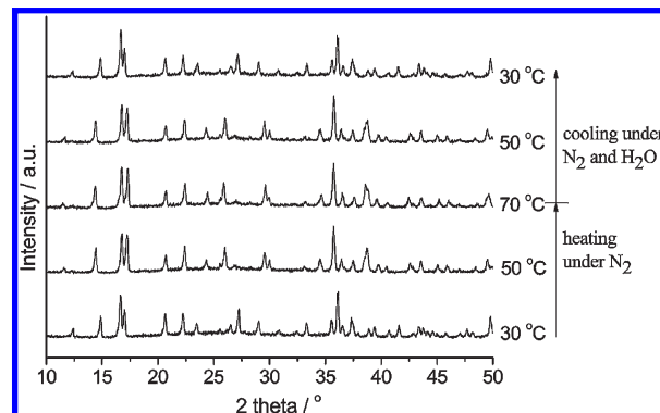
Figure 2. In situ variable-temperature powder XRD patterns of Tb(H 2 O) 5 [W(CN) 8 ] with desorption and resorption of one coordinated water molecule.
