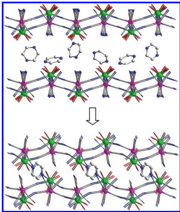
Figure 4. 2D-Corrugated layers 17f further pillared by pyrazine ligands in the presence of heat, resulting in the formation of a 3D heterometallic network of 1 .
