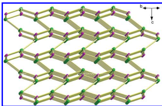
Figure 5. Topological representation of the 3D framework of 1 .
