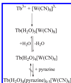
Scheme 1. Formation Mechanism of 1
