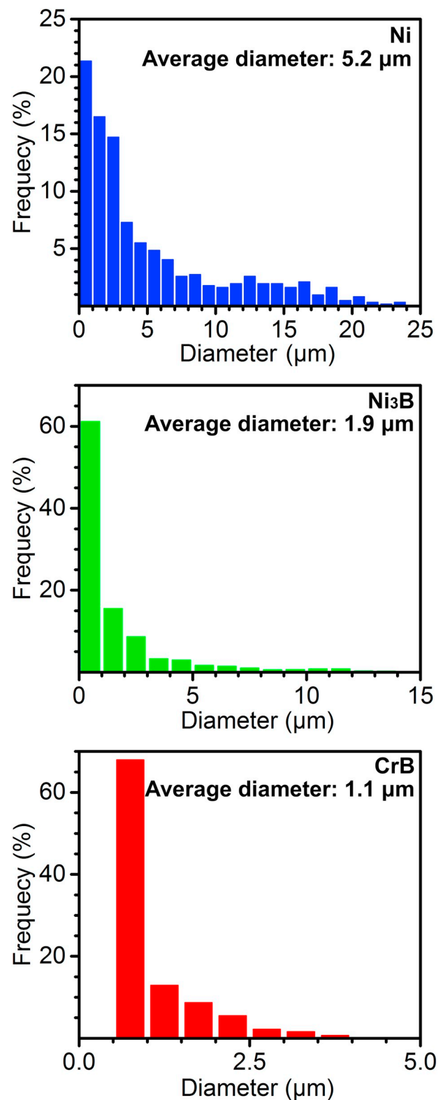
Fig. 6. Size distributions of the Ni, Ni 3 B and CrB grains in the remelted NiCrBSi coating.
