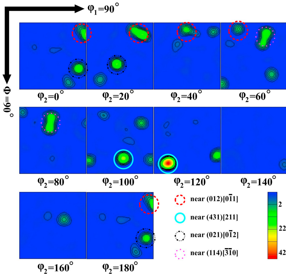
Fig. 10. Selected orientation distribution functions of the \text{Ni}_3\text{B} grains in the remelted NiCrBSi coating.
