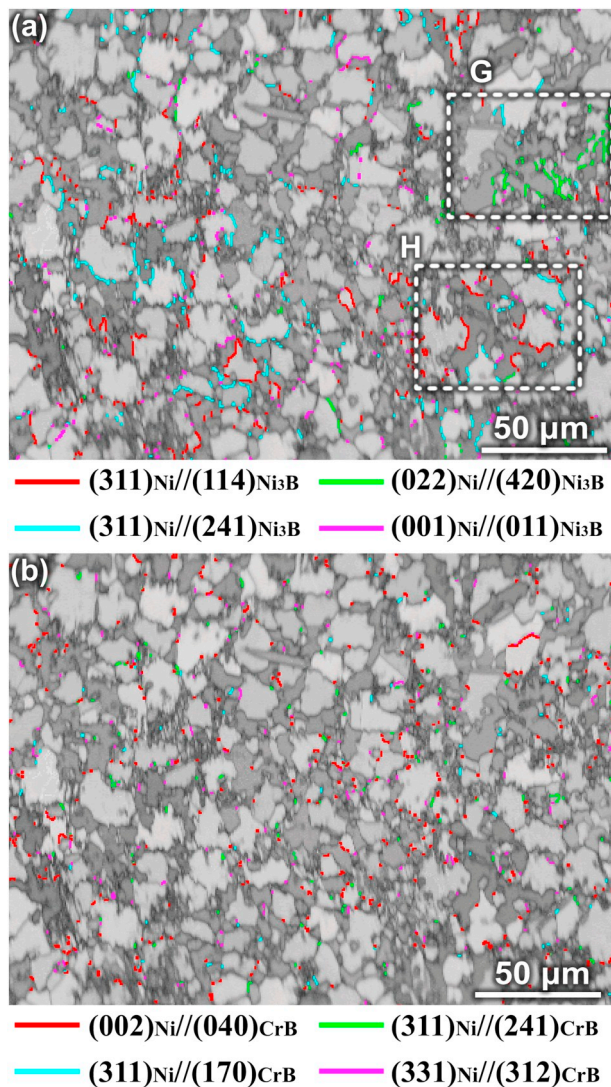
Fig. 13. Selected lattice correlation boundaries represented by different colors: (a) between the adjacent Ni and \text{Ni}_3\text{B} grains, (b) between the adjacent Ni and CrB grains. The dash rectangles G and H in (a) contain two independent \text{Ni}_3\text{B} colonies.
