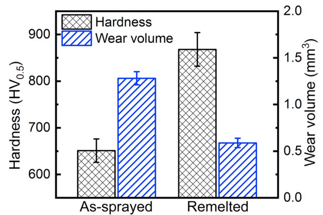
Fig. 2. Hardness and wear volume of the as-sprayed and remelted NiCrBSi coatings.
