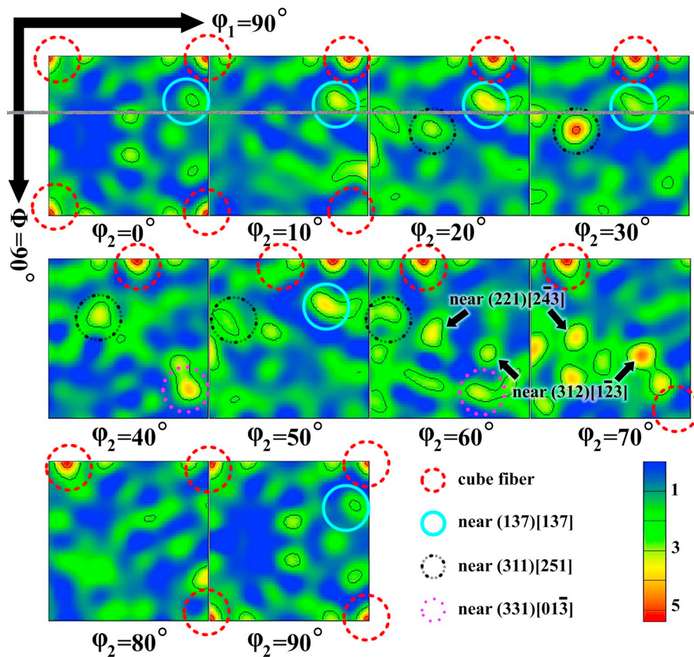
Fig. 8. Selected orientation distribution functions of the Ni grains in the NiCrBSi remelted coating.
