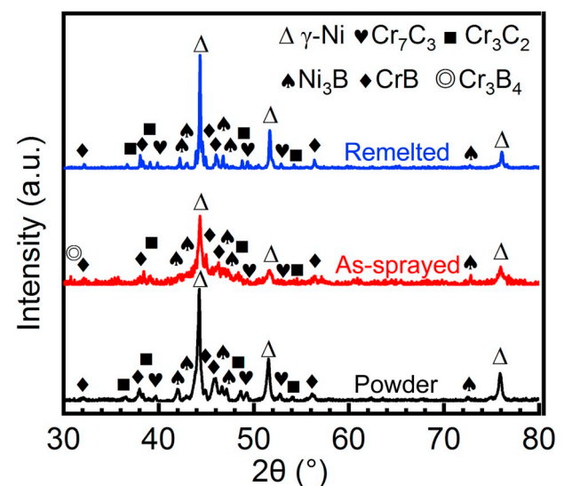
Fig. 3. XRD patterns of the raw powder, the as-sprayed and remelted NiCrBSi coatings.
