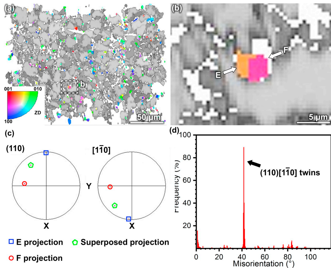
Fig. 11. EBSD results of the remelted NiCrBSi coating: (a) inverse pole figure map for CrB grains, (b) magnified image of the dash rectangle region b in (a), (c) the (110) and [1\bar{1}0] pole figures of E and F parts marked in (b), (d) misorientation angle distribution histogram of the neighboring Ni grains.
