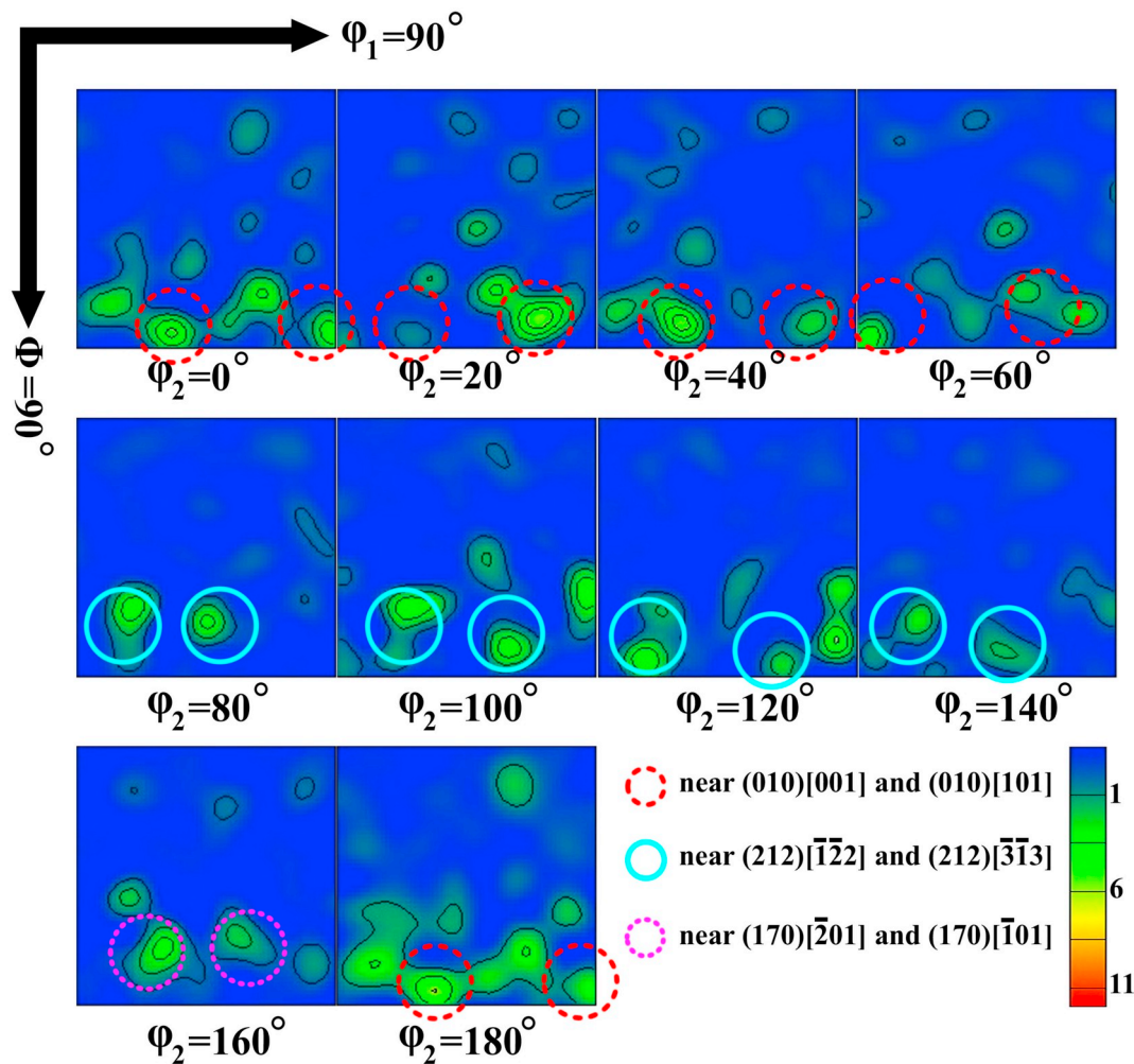
Fig. 12. Selected orientation distribution functions of the CrB grains in the remelted NiCrBSi coating.
