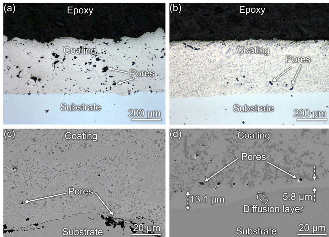
Fig. 4. Cross-sectional microstructures of the coatings: optical microscopy images for (a) as-sprayed and (b) remelted NiCrBSi coatings and scanning electrons microscopy image for (c) as-sprayed and (d) remelted NiCrBSi coatings.
