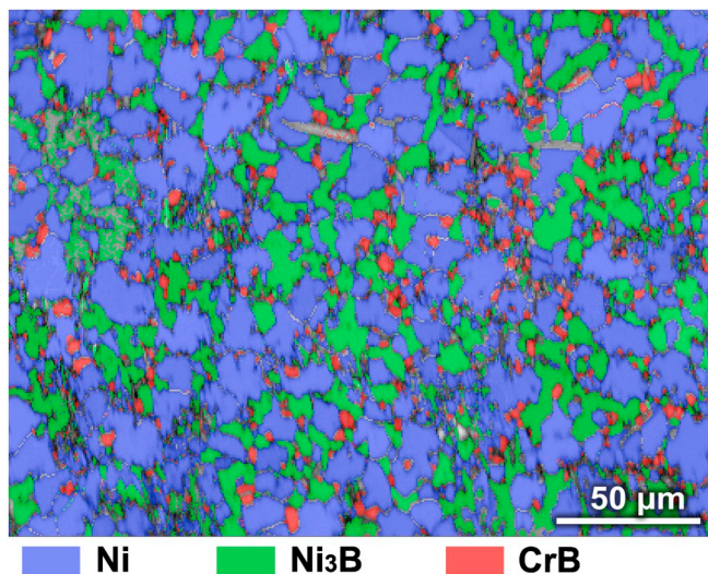
Fig. 5. Grain color map of the remelted NiCrBSi coating.
