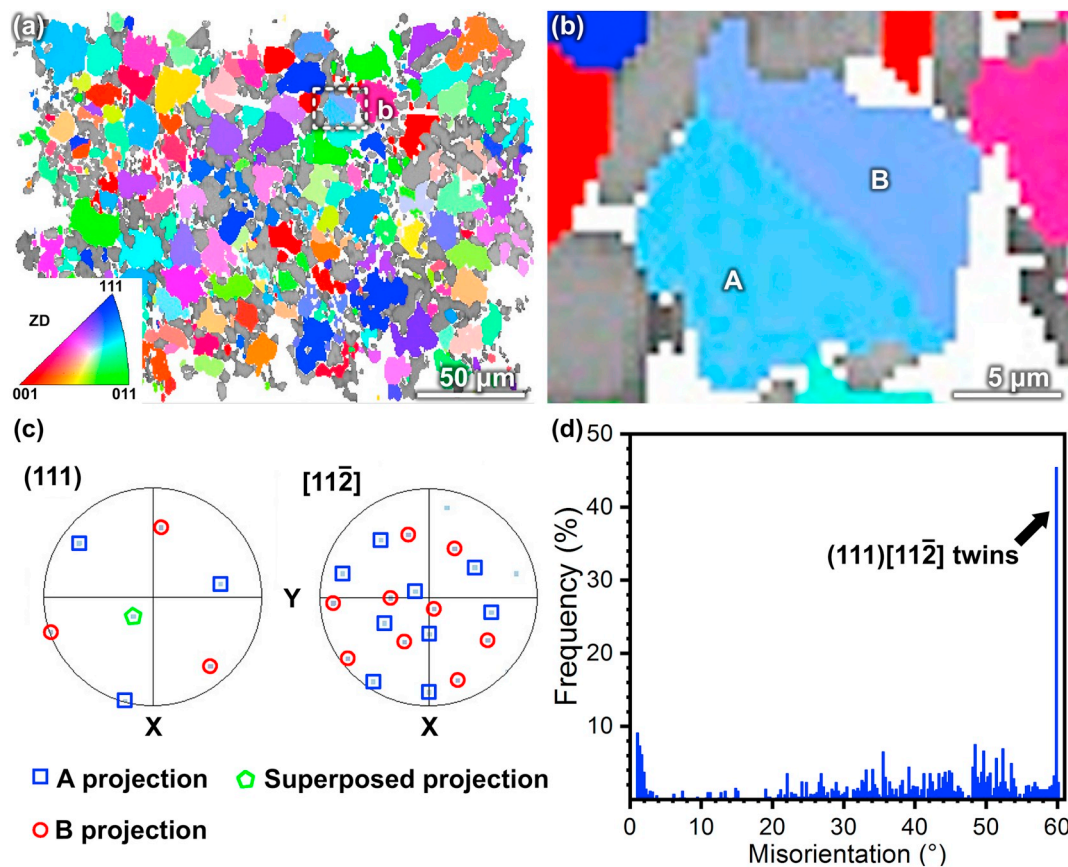
Fig. 7. EBSD results of the remelted NiCrBSi coating: (a) inverse pole figure map for Ni grains, (b) magnified image of the dash rectangle region b in (a), (c) the (111) and [11\bar{2}] pole figures of A and B parts marked in (b), (d) misorientation angle distribution histogram of the neighboring Ni grains.
