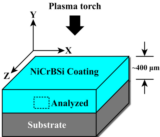
Fig. 1. Schematic interpretation of the coordinate axes of the remelted NiCrBSi coating sample in EBSD characterization.
