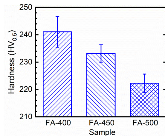
Figure 4. Hardness of the samples after final annealing.
